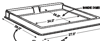
Drainless Base WMPBD27 or WMPBD32
